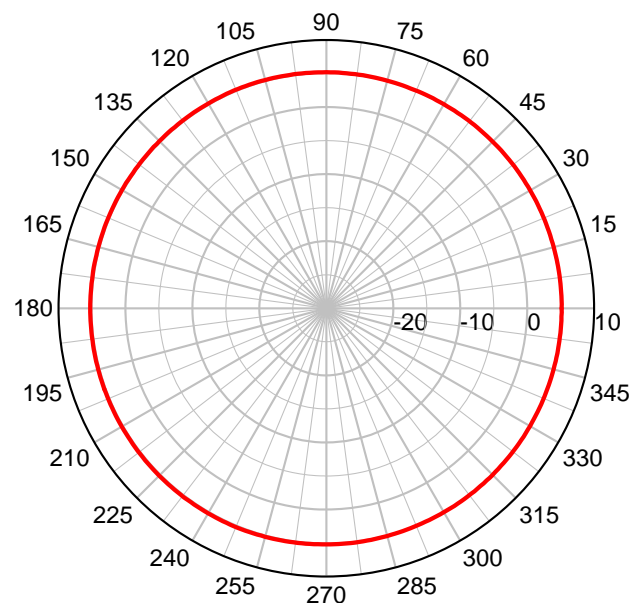
MGD @ 5500 MHz-Azimuth
