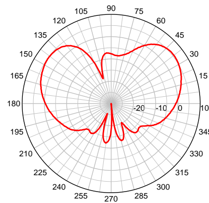
SMW 2400 MHz – Elevation Plot
