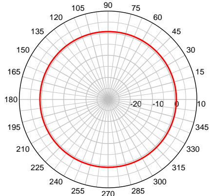
SMW 700 MHz – Azimuth Plot
