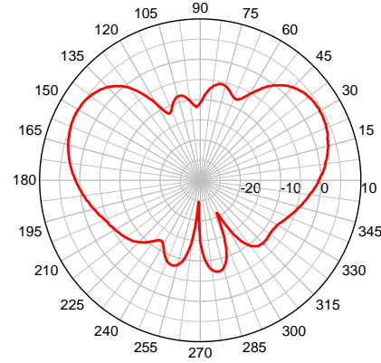
SMW 1900 MHz- Elevation Plot
