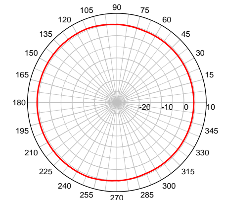
SMW 5500 MHz – Azimuth Plot
