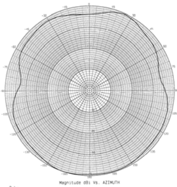
2450 MHz – Azimuth
