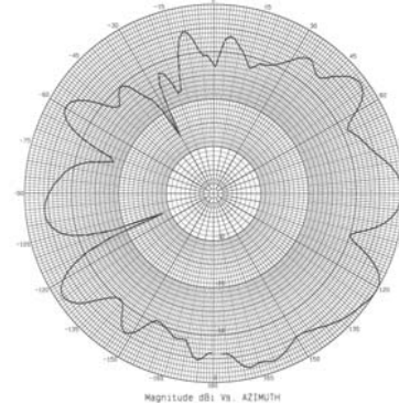
5500 MHz – Azimuth
