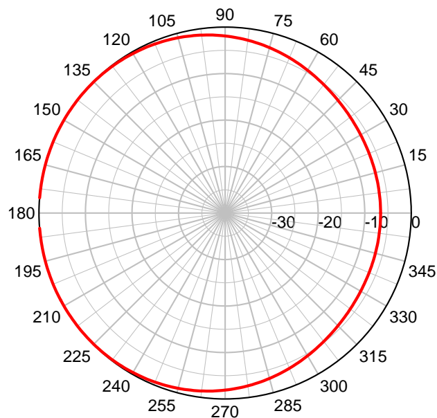
ODR-2400K – Azimuth Plot
