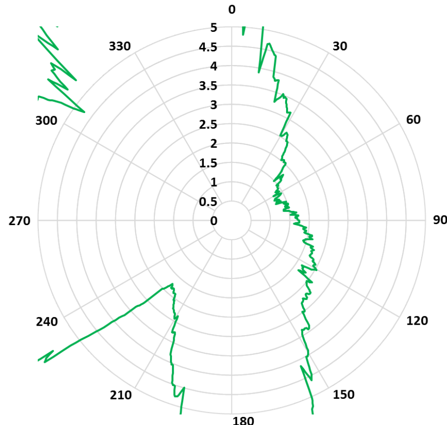
867 MHz Azimuth Axial Ratio Plot
