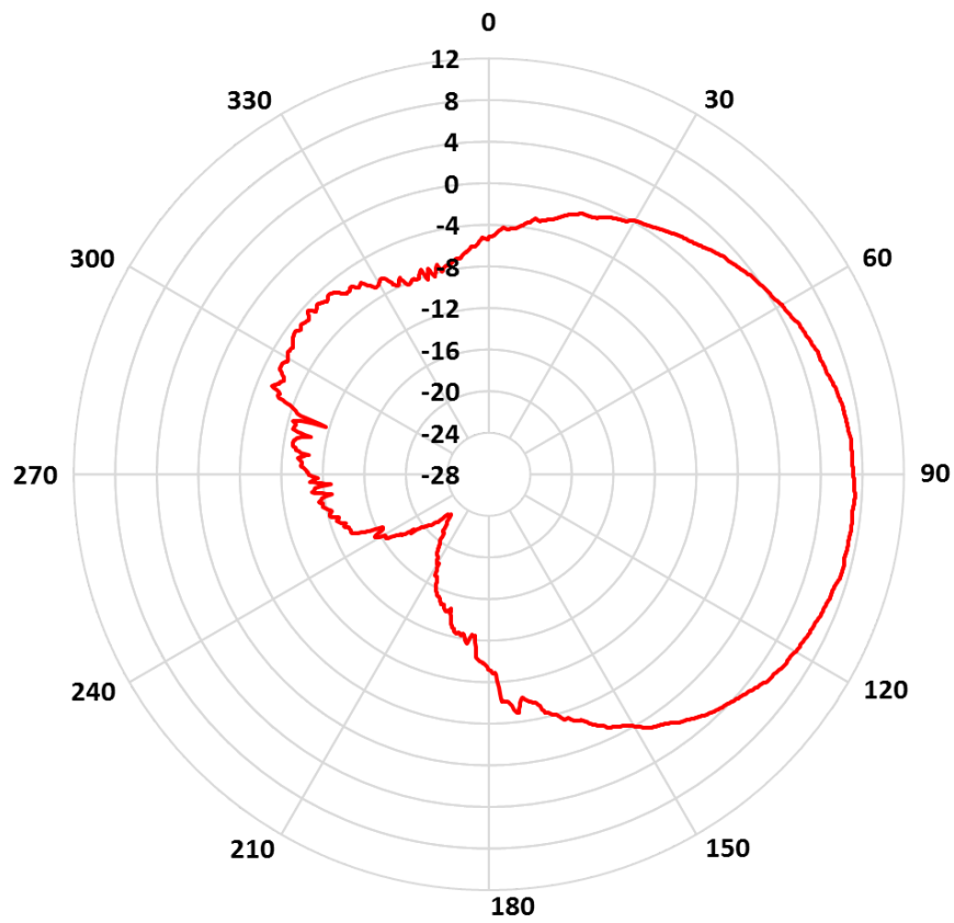
867 MHz Azimuth Gain Plot
