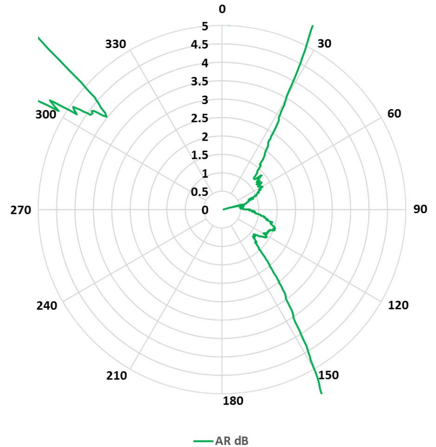
910 MHz Azimuth Axial Ratio Plot
