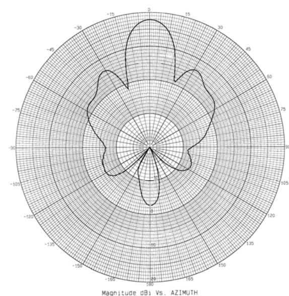
PN16-3000 @ 3.5 GHz – Azimuth Plot
