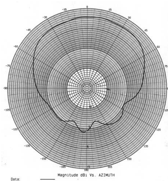
PS10-3500-120 – Azimuth Plot
