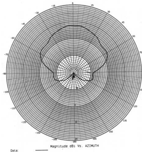
PS12-5500-60 – Azimuth Plot
