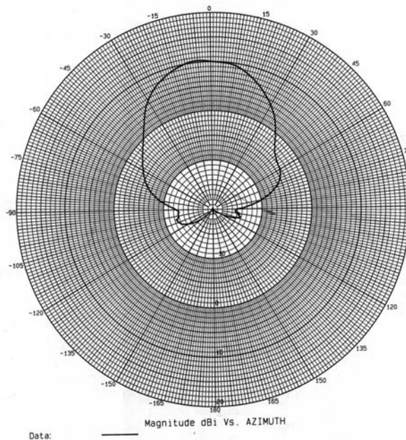
PS14-5900-45 Azimuth Plot
