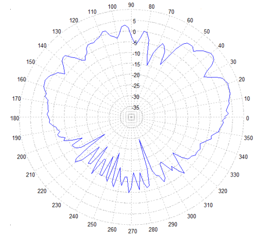
5500 MHz – Elevation Plot
