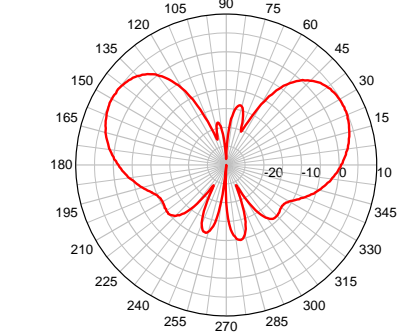
RMM 1800 MHz – Elevation Plot
