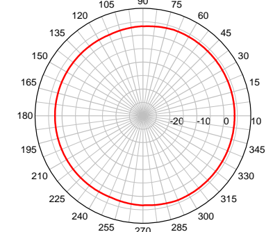
RMM 2400 MHz – Azimuth Plot
