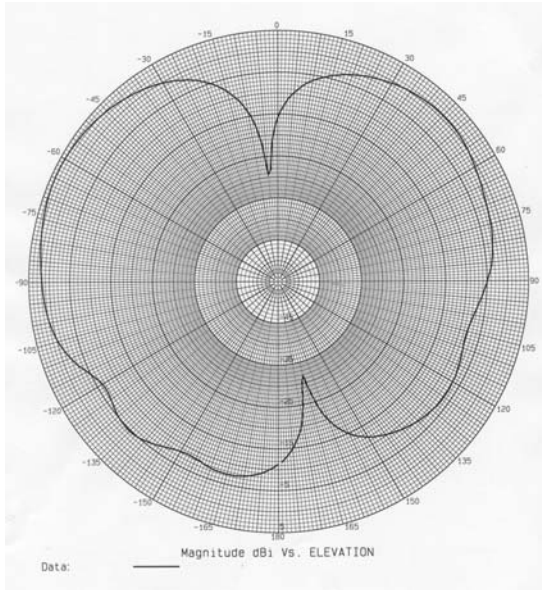
SMD @ 2500 MHz – Elevation Plot
