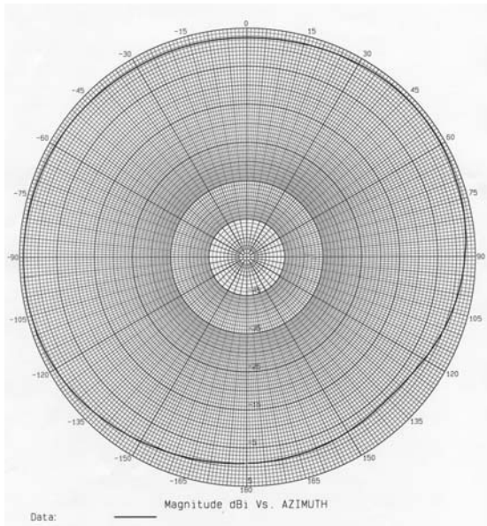
SMD @ 2500 MHz – Azimuth Plot
