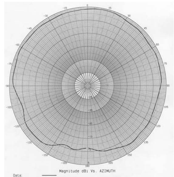
SMD @ 5500 MHz- Azimuth Plot
