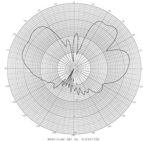
5950 MHz – Elevation Plot
