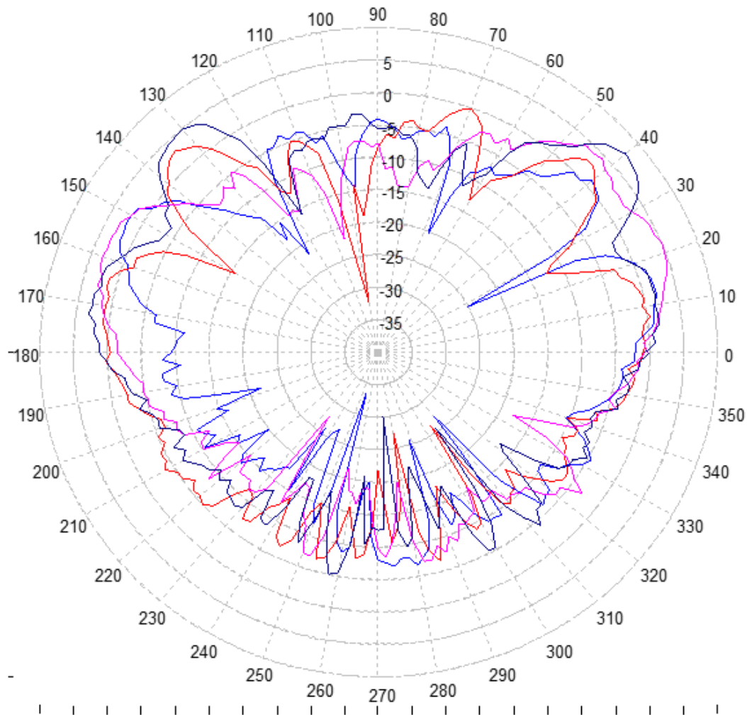
5900 MHz – Elevation Plot – 4cuts
