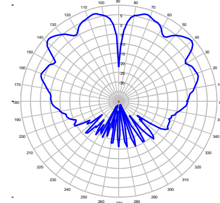
6000 MHz – Elevation Plot
