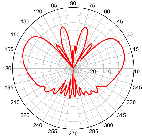
DM2 5500 Series – Elevation Plot
