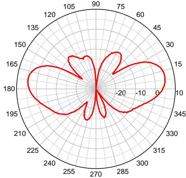
IMAG5-2400 – Elevation Plot
