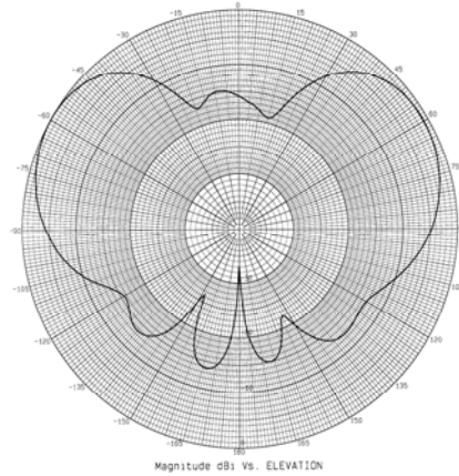
1850 MHz – Elevation Plot
