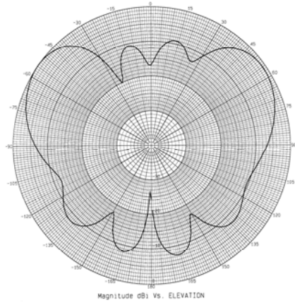
1750 MHz – Elevation Plot
