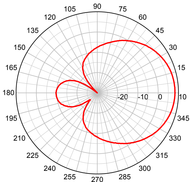
P8S-2400 – Azimuth Plot
