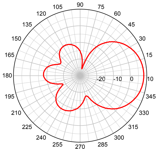
P8S-2400 – Elevation Plot
