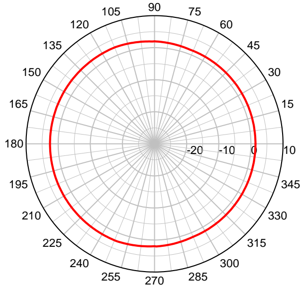
PSKN3-1900S Series – Azimuth Plot
