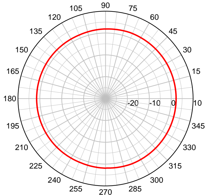
PSKN3 925S Series – Azimuth Plot
