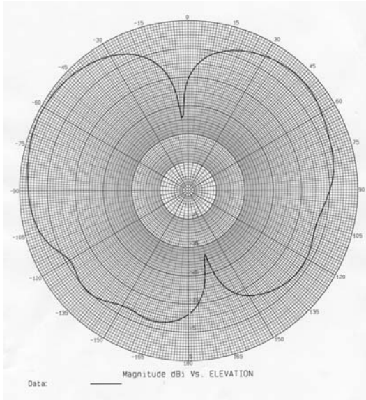
SMD @ 2500 MHz – Elevation Plot
