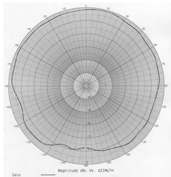
SMD @ 5500 MHz – Azimuth Plot
