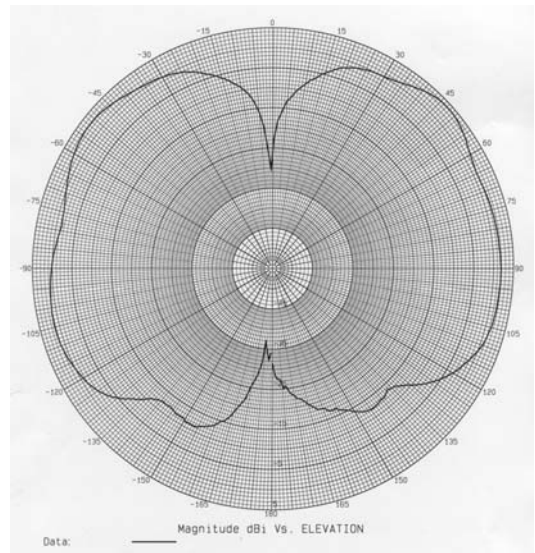
SMD @ 5500 MHz – Elevation Plot
